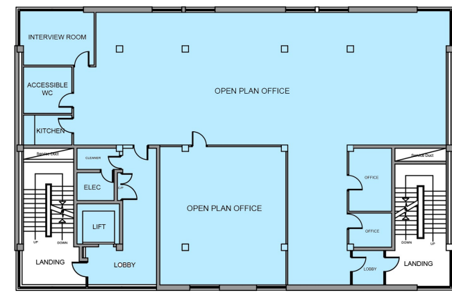
SIXTH FLOOR
