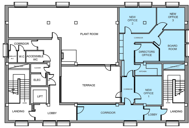
SEVENTH FLOOR
